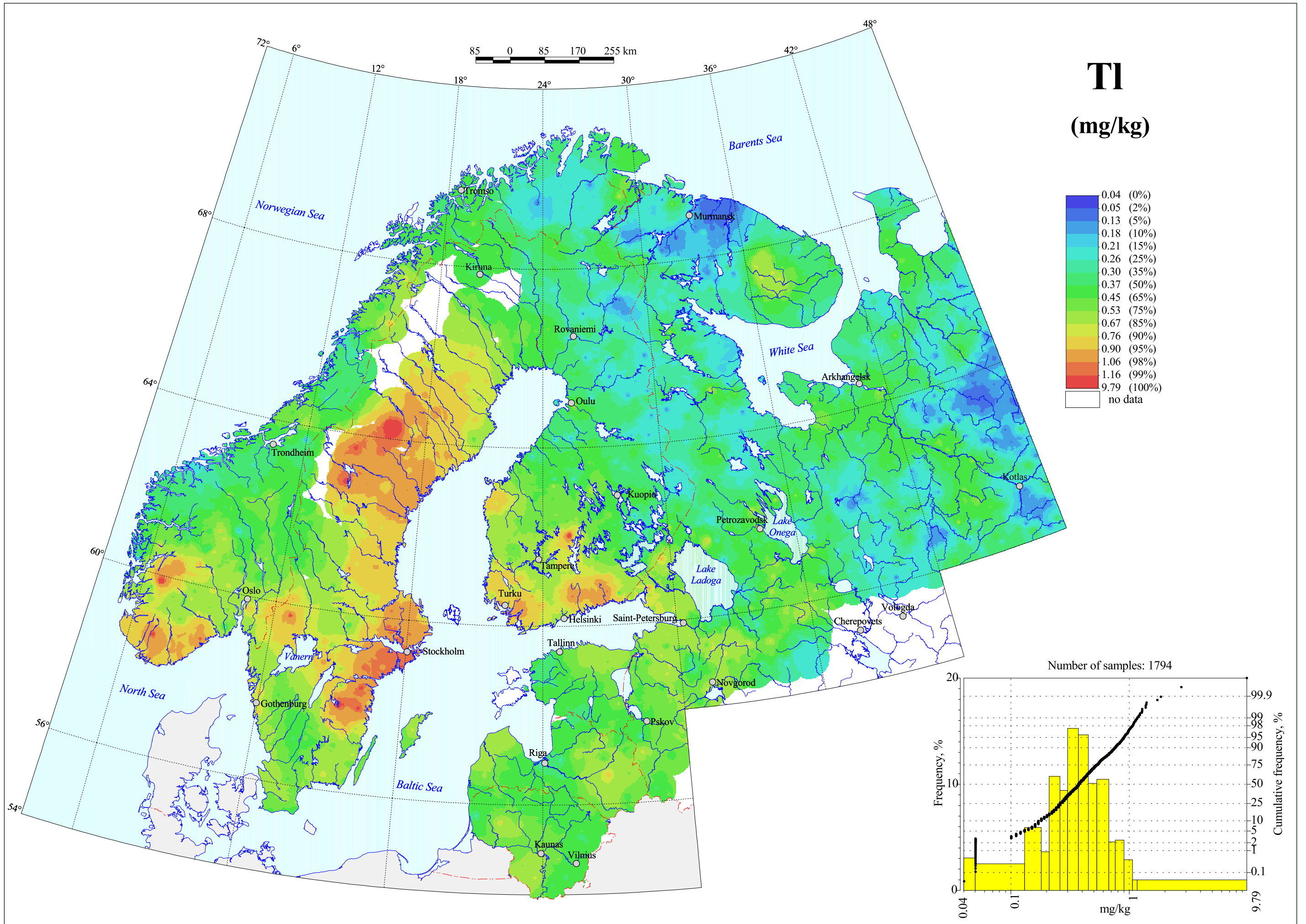
Thallium in C-horizon, Grain Size <2 mm, Total Content
